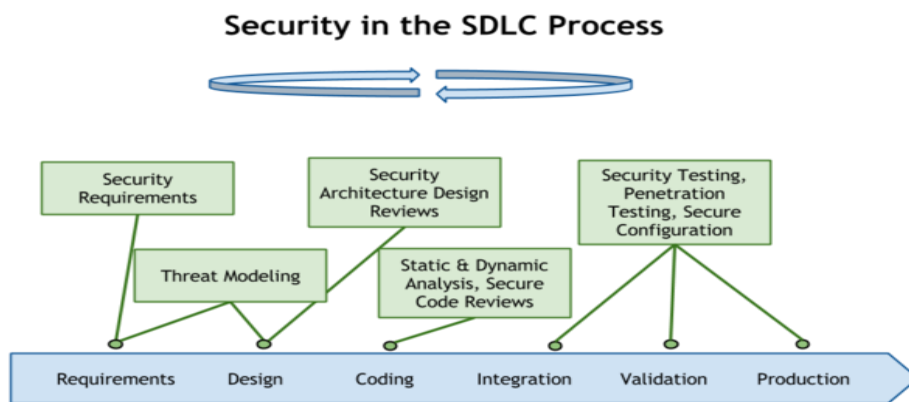
Fig. 1: Security integration in SDLC
