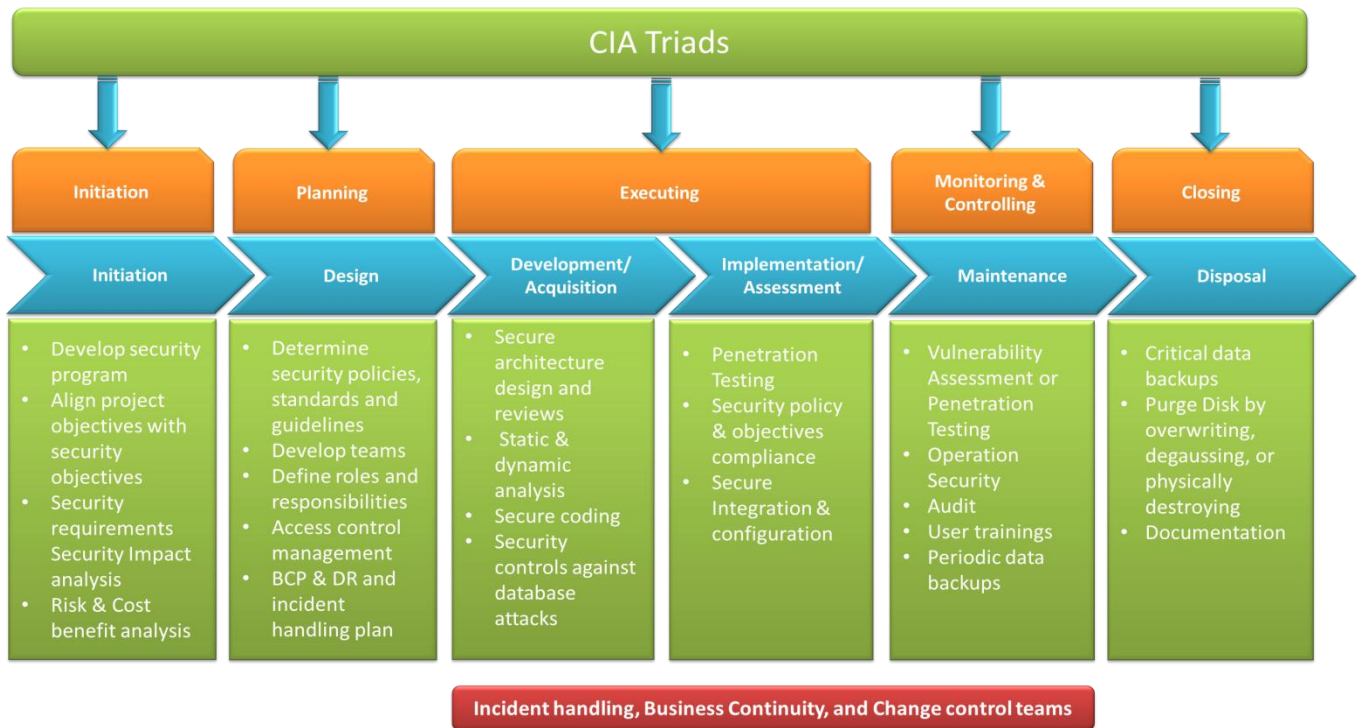
Fig. 3: ITPMS (IT project management security) Proposed Framework
