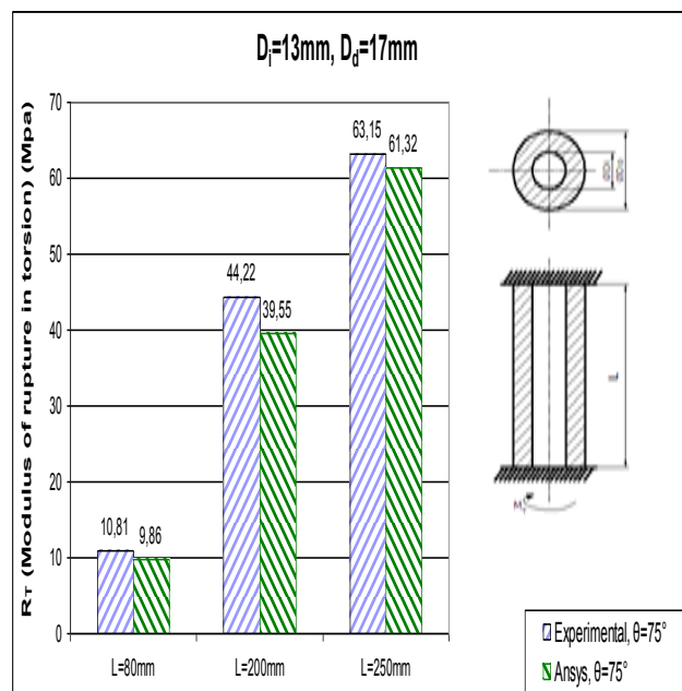
Fig. 6 Effects of length of specimens for carbon/epoxy on torsion stress
