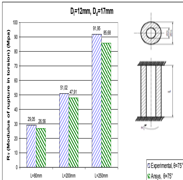
Fig. 5 Effects of length of specimens for carbon/epoxy on torsion stress
